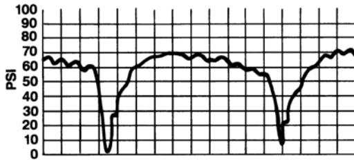
1" PUMP WITHOUT SHOCK BLOCKER (From lower chart at right)
